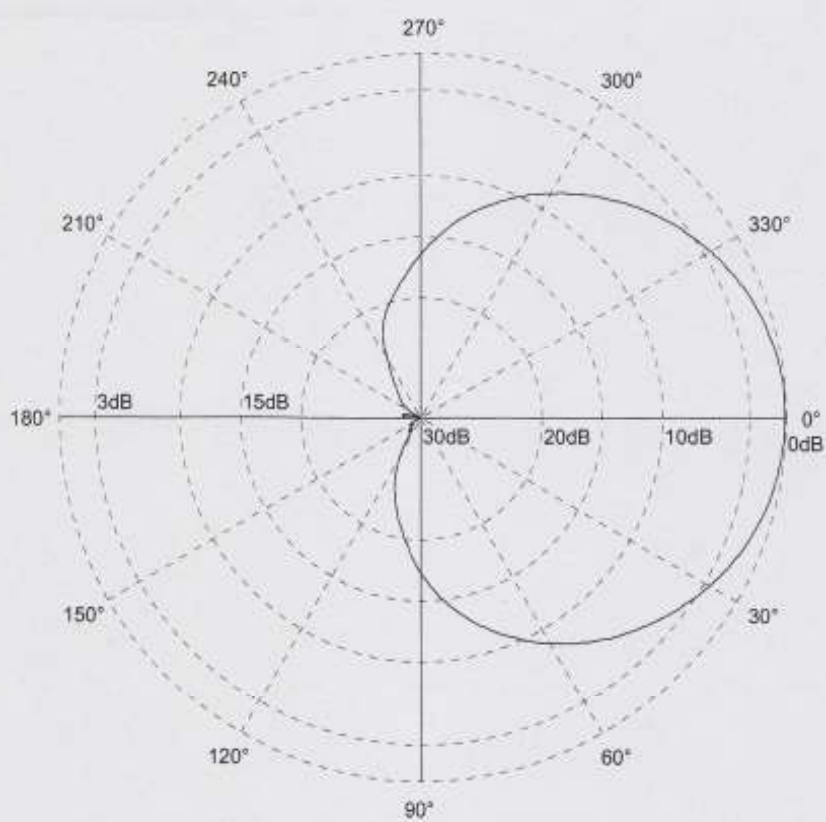
Horizontal Radiation Pattern
